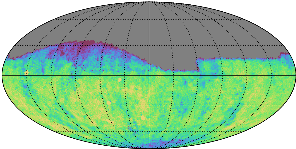
ddf_acor_sf10_lsf20_lsr20_v3.4_10yrs Yr 1 g band: CoaddM5
