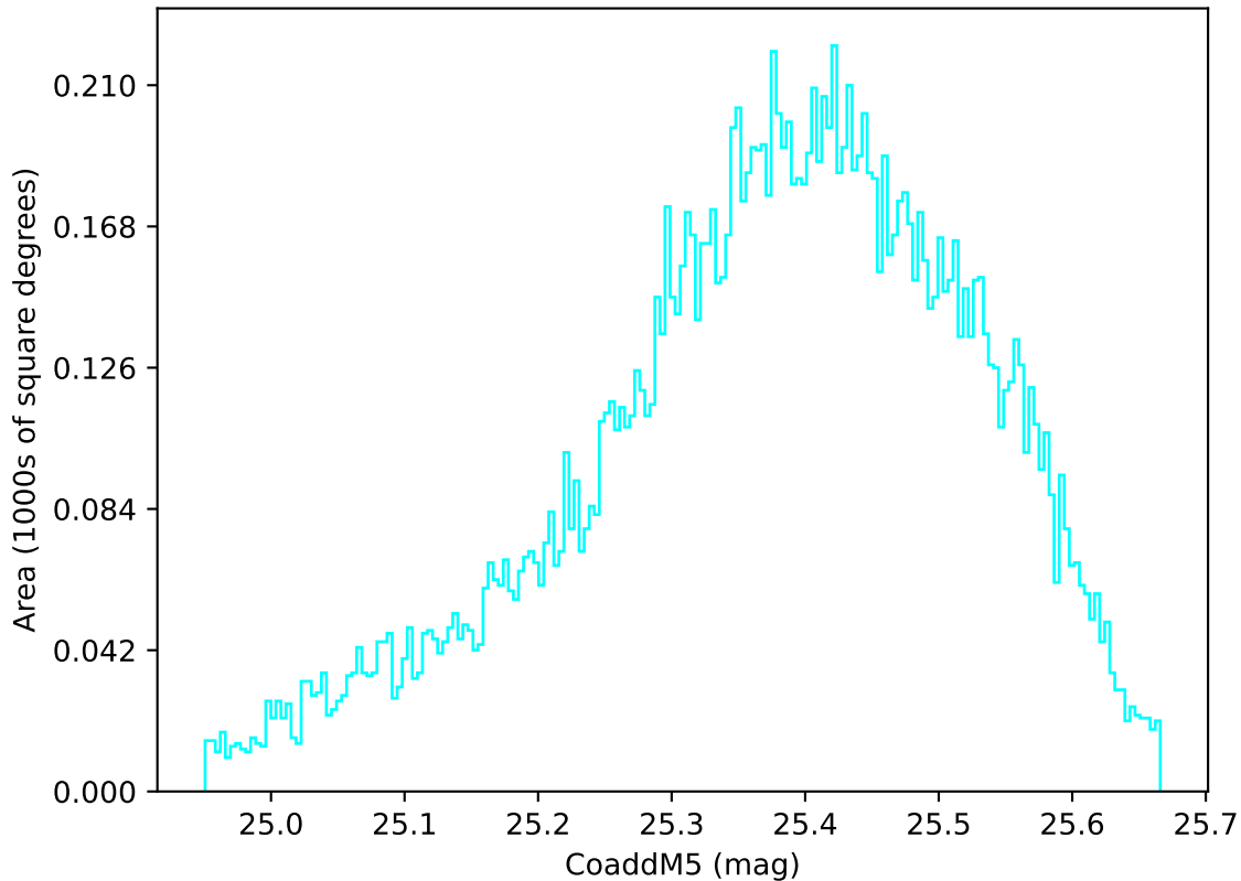
ddf_acor_sf10_lsf20_lsr20_v3.4_10yrs WFD u band: CoaddM5
