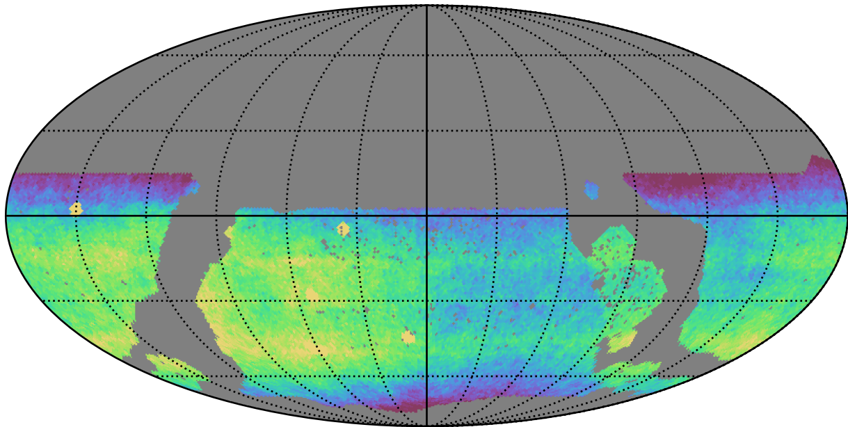
ddf_acor_sf10_lsf20_lsr20_v3.4_10yrs WFD r band: CoaddM5
