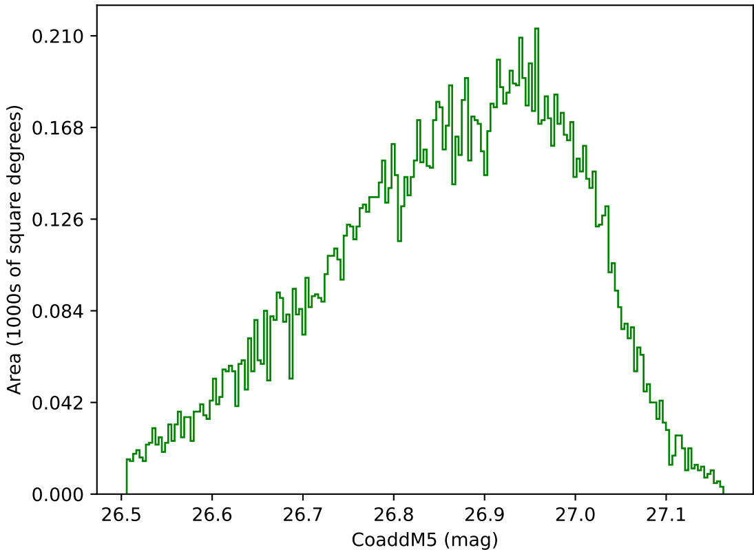
ddf_acor_sf10_lsf20_lsr20_v3.4_10yrs WFD g band: CoaddM5
