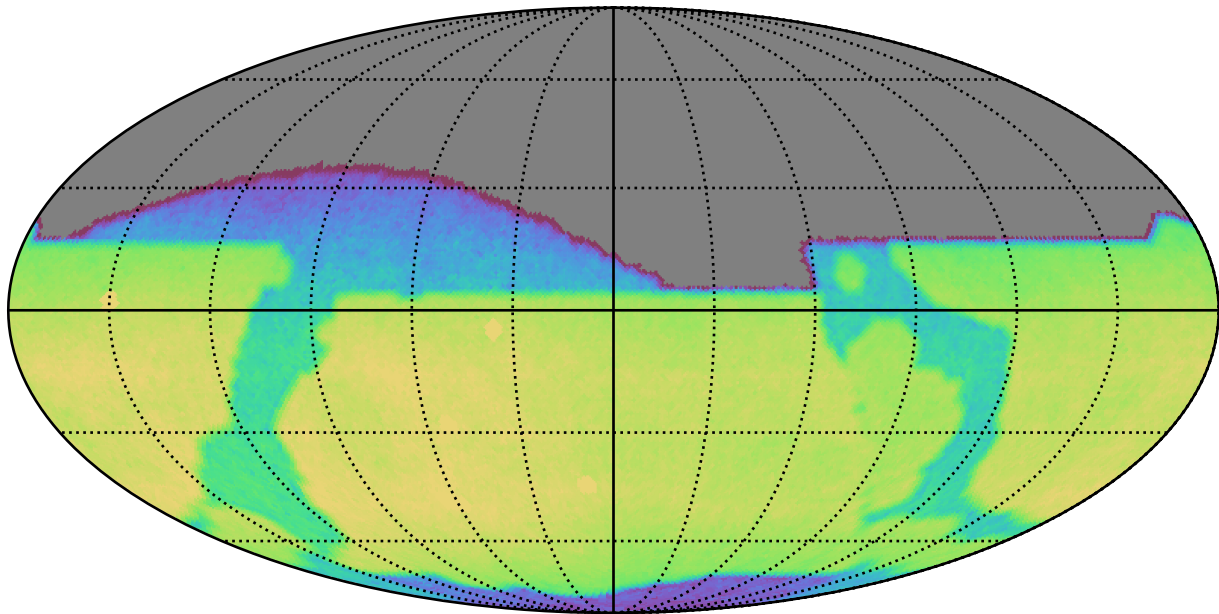
ddf_acor_sf10_lsf20_lsr20_v3.4_10yrs All sky z band: CoaddM5
