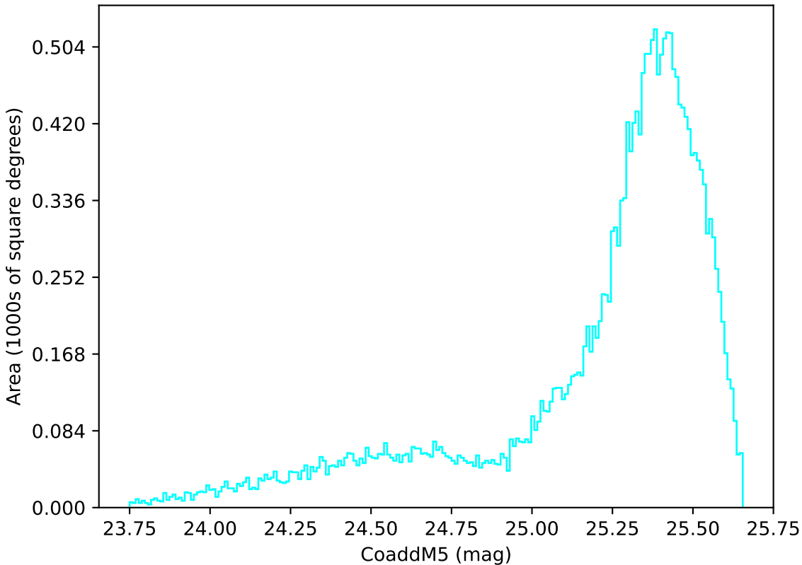
ddf_acor_sf10_lsf20_lsr20_v3.4_10yrs All sky u band: CoaddM5
