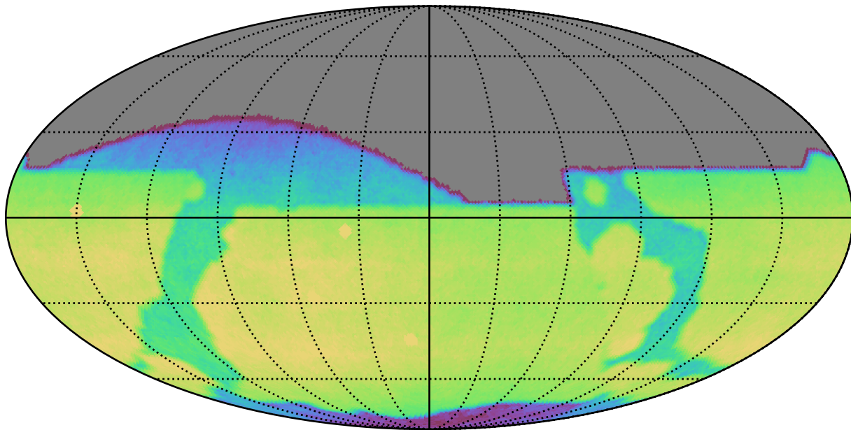
ddf_acor_sf10_lsf20_lsr20_v3.4_10yrs All sky r band: CoaddM5
