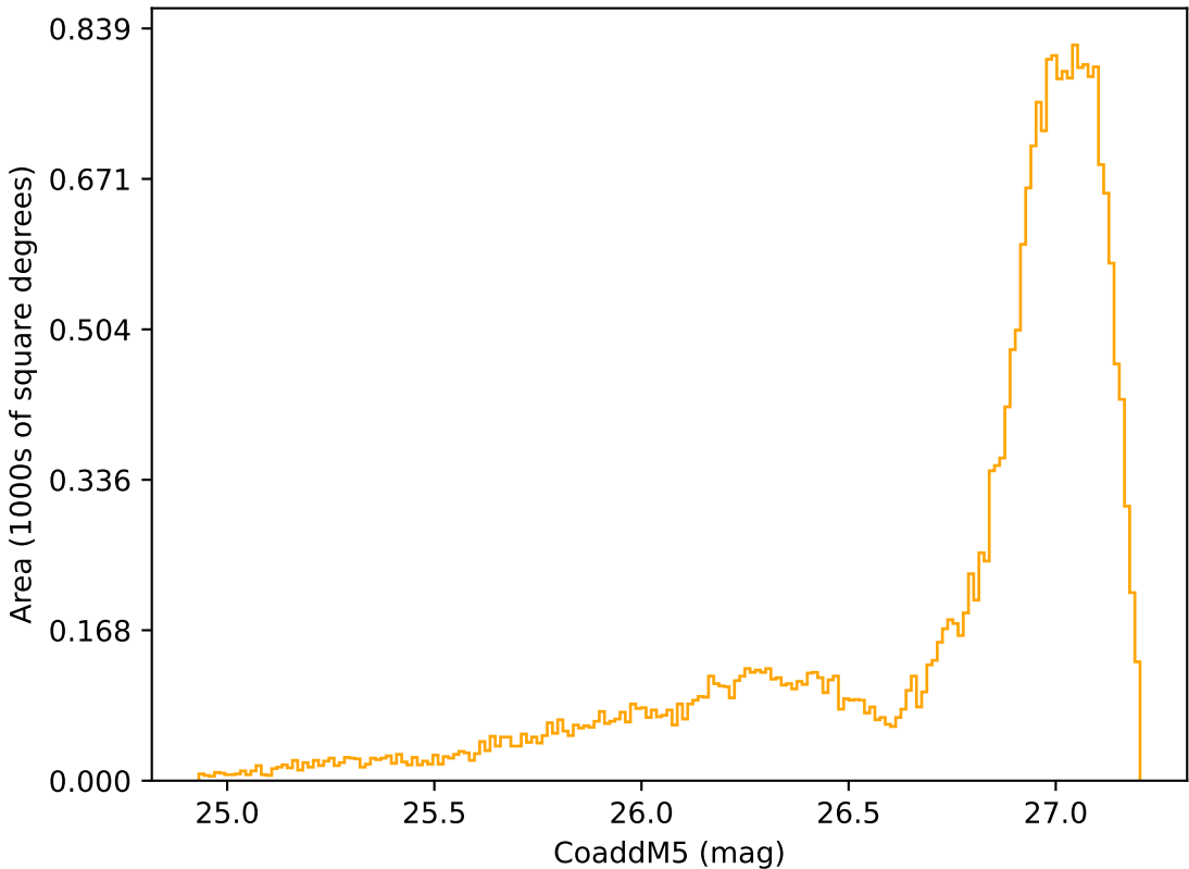
ddf_acor_sf10_lsf20_lsr20_v3.4_10yrs All sky r band: CoaddM5
