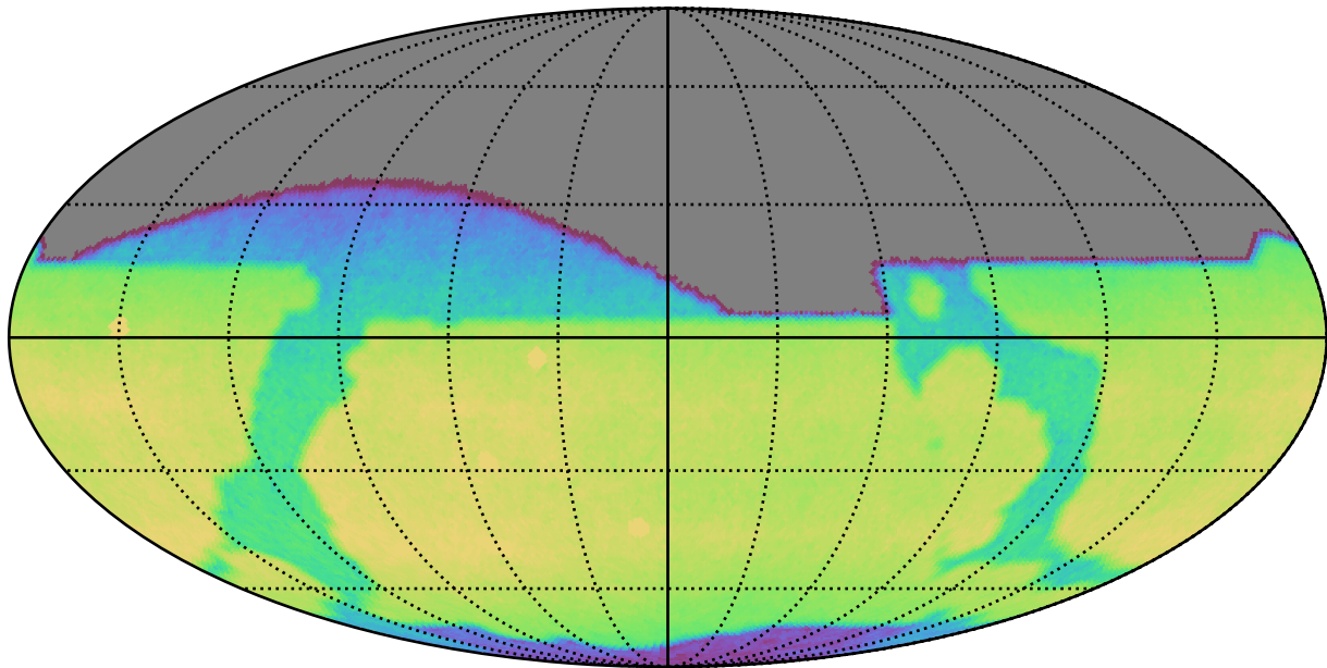
ddf_acor_sf10_lsf20_lsr20_v3.4_10yrs All sky i band: CoaddM5
