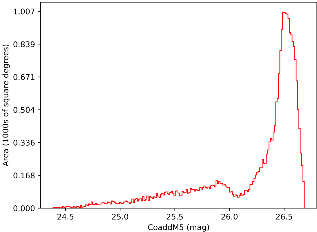
ddf_acor_sf10_lsf20_lsr20_v3.4_10yrs All sky i band: CoaddM5
