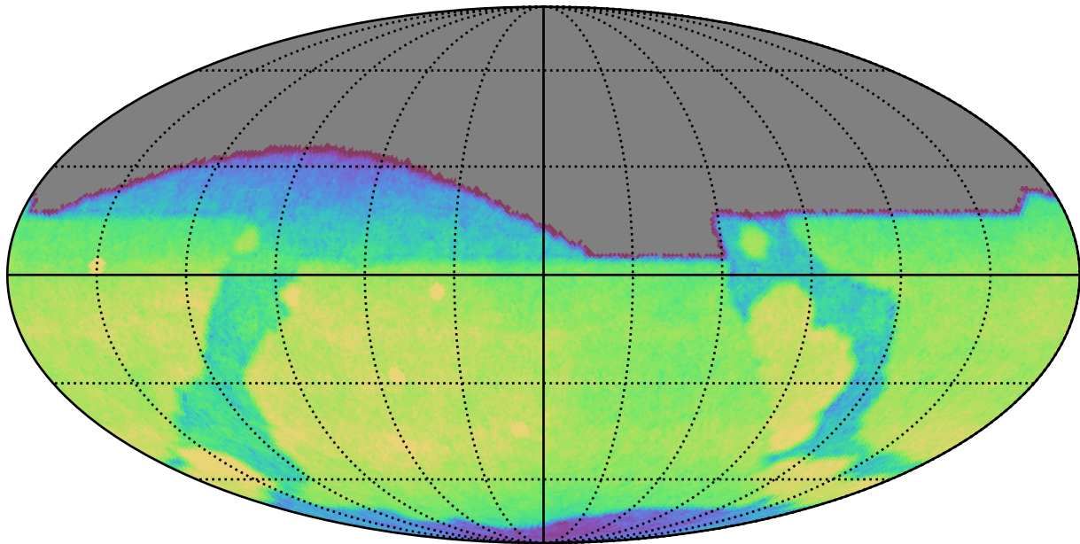
ddf_acor_sf10_lsf20_lsr20_v3.4_10yrs All sky g band: CoaddM5
