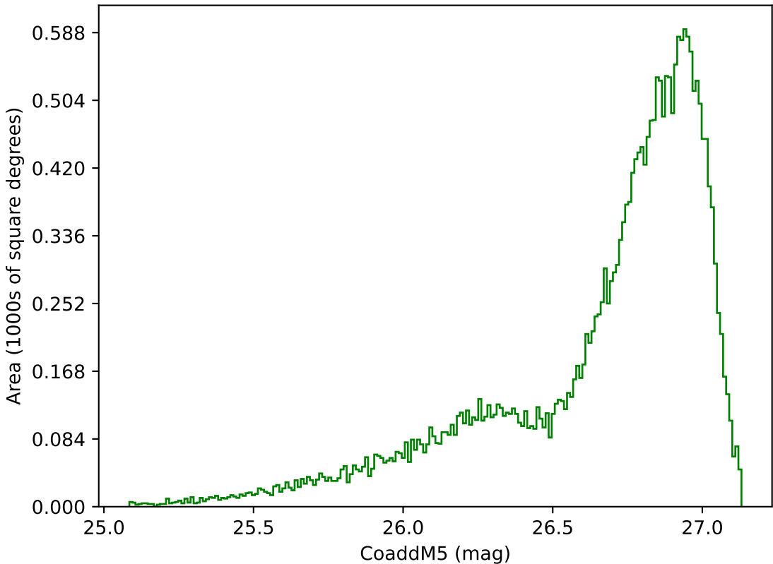
ddf_acor_sf10_lsf20_lsr20_v3.4_10yrs All sky g band: CoaddM5
