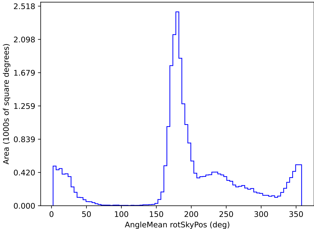
ddf_acor_sf10_lsf20_lsr20_v3.4_10yrs All sky r band: AngleMean rotSkyPos
