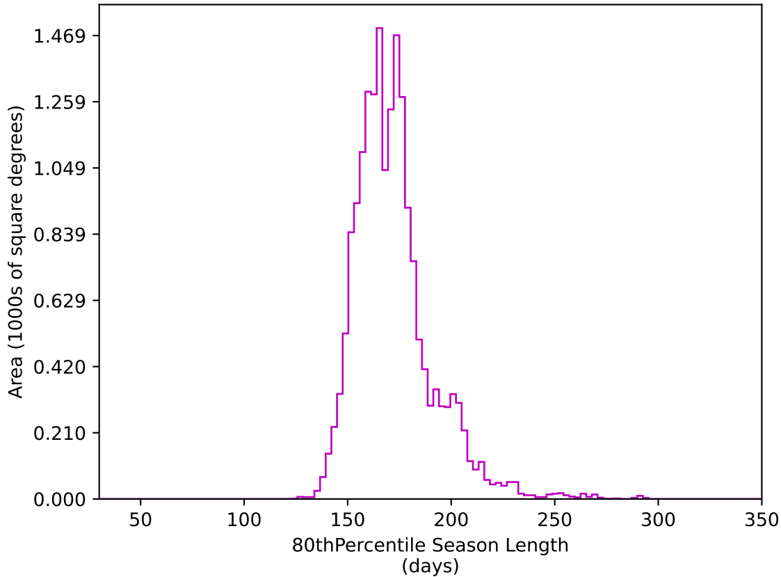
ddf_acor_sf10_lsf20_lsr20_v3.4_10yrs WFD z band: 80thPercentile Season Length
