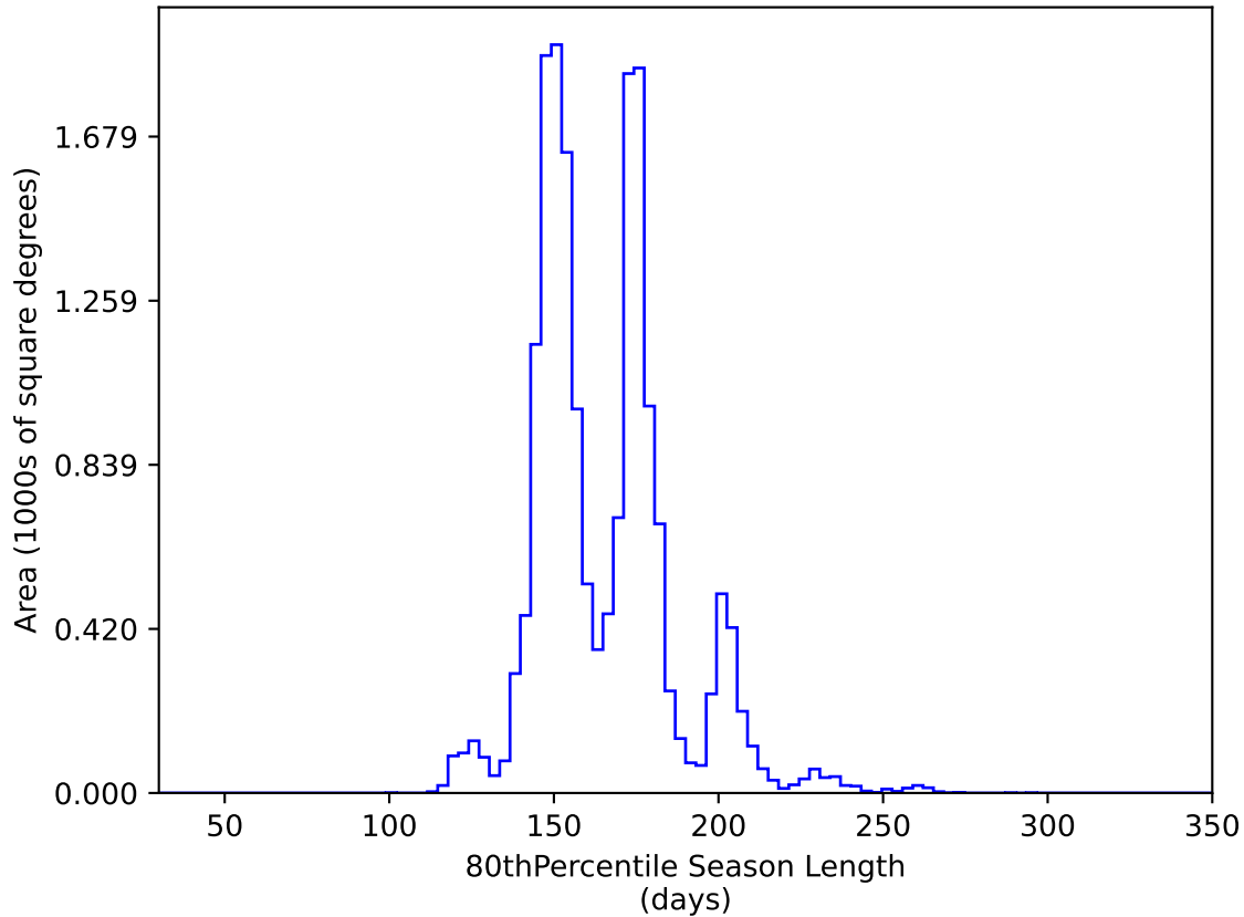
ddf_acor_sf10_lsf20_lsr20_v3.4_10yrs WFD y band: 80thPercentile Season Length
