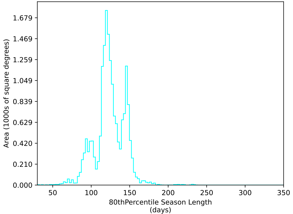
ddf_acor_sf10_lsf20_lsr20_v3.4_10yrs WFD u band: 80thPercentile Season Length
