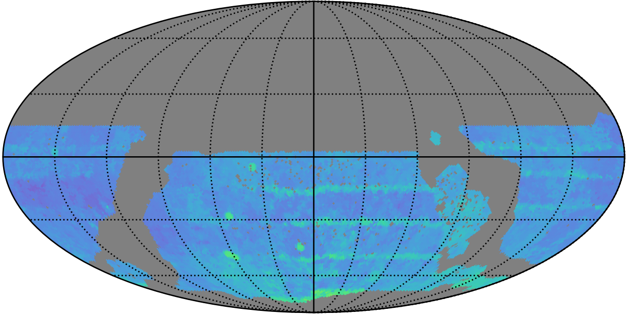
ddf_acor_sf10_lsf20_lsr20_v3.4_10yrs WFD r band: 80thPercentile Season Length
