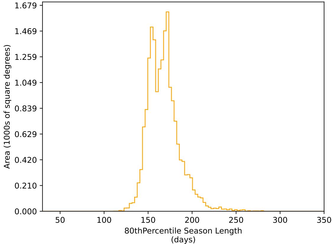
ddf_acor_sf10_lsf20_lsr20_v3.4_10yrs WFD r band: 80thPercentile Season Length
