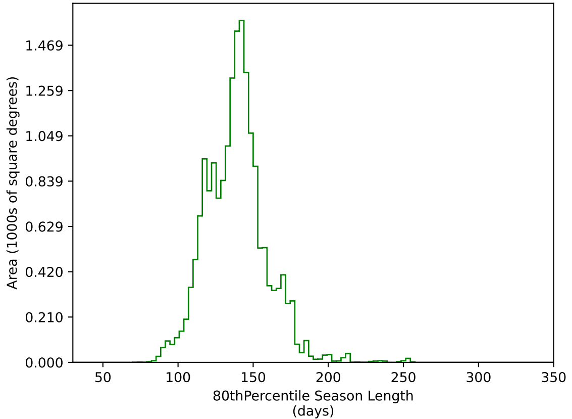
ddf_acor_sf10_lsf20_lsr20_v3.4_10yrs WFD g band: 80thPercentile Season Length
