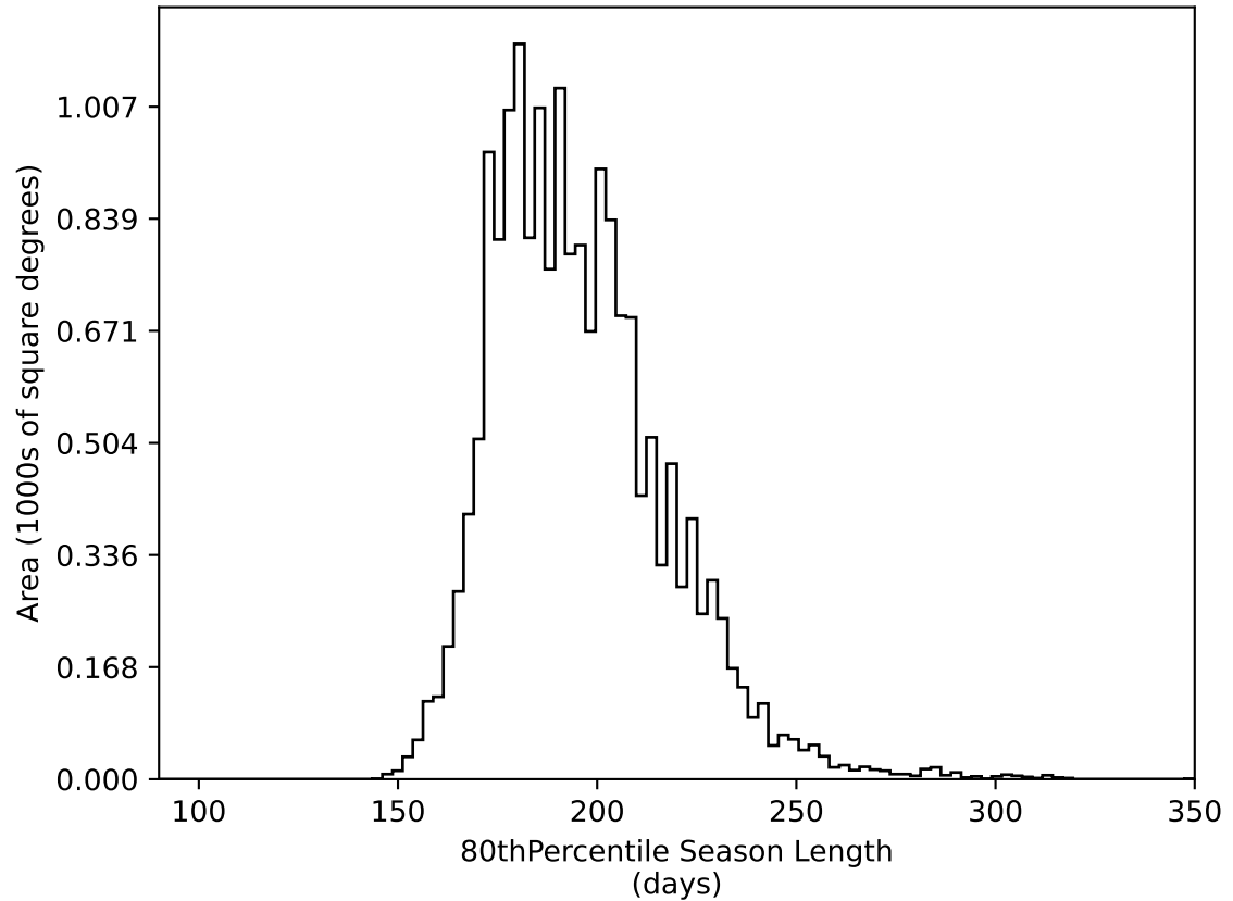
ddf_acor_sf10_lsf20_lsr20_v3.4_10yrs WFD all bands: 80thPercentile Season Length
