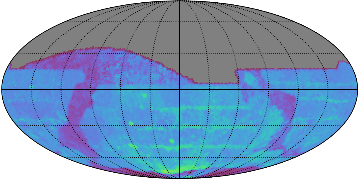
ddf_acor_sf10_lsf20_lsr20_v3.4_10yrs All sky z band: 80thPercentile Season Length
