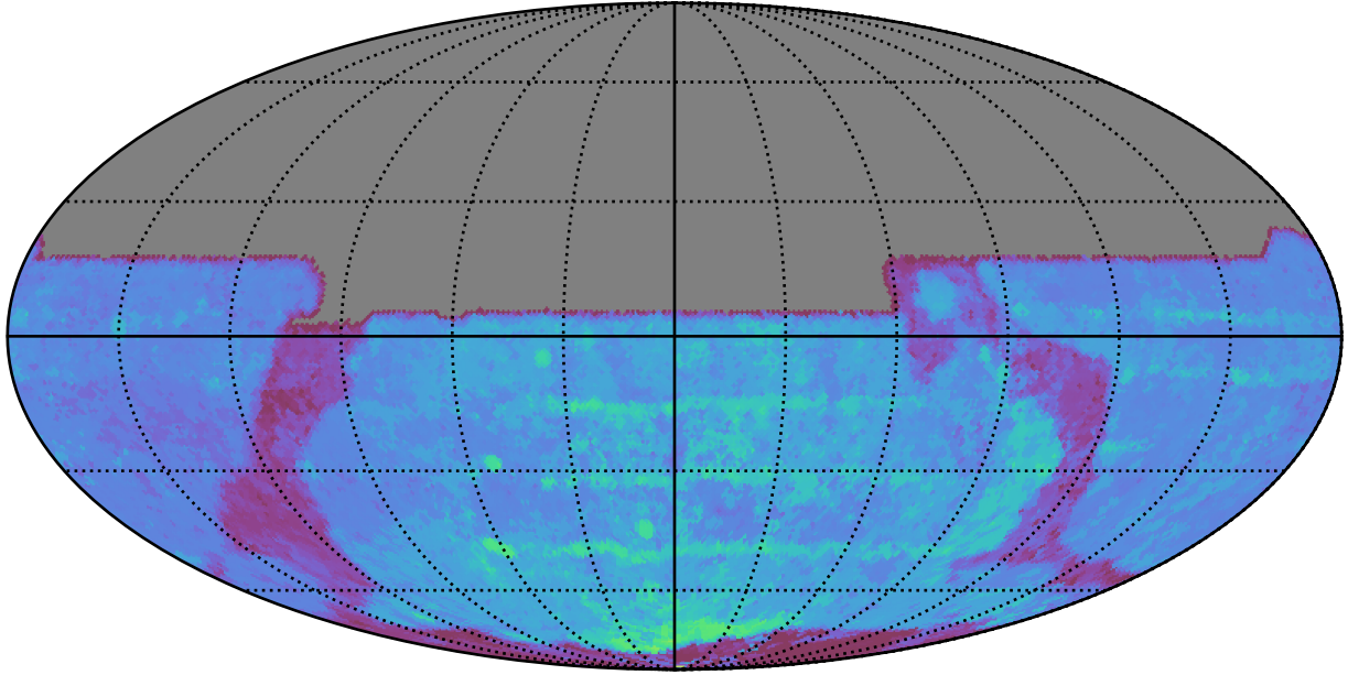
ddf_acor_sf10_lsf20_lsr20_v3.4_10yrs All sky y band: 80thPercentile Season Length
