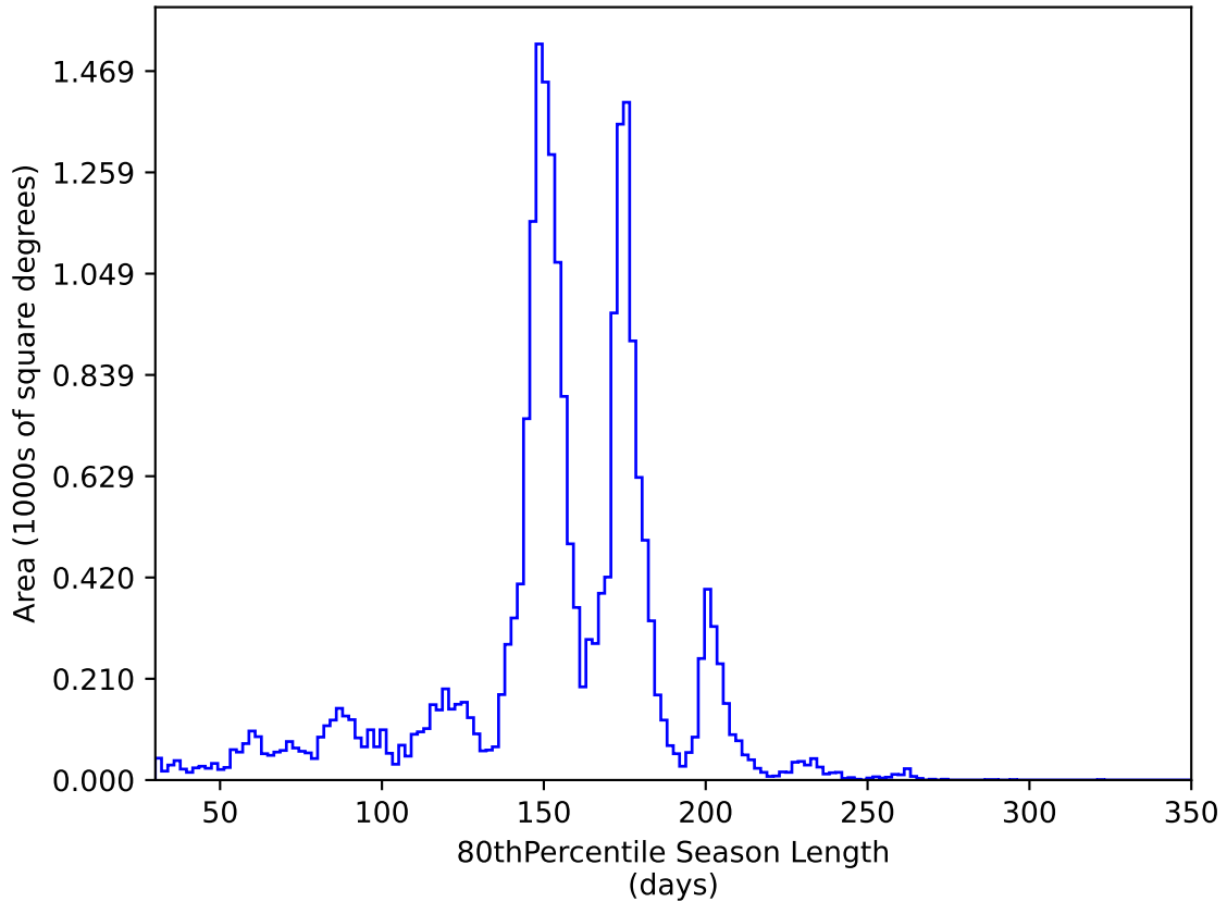
ddf_acor_sf10_lsf20_lsr20_v3.4_10yrs All sky y band: 80thPercentile Season Length
