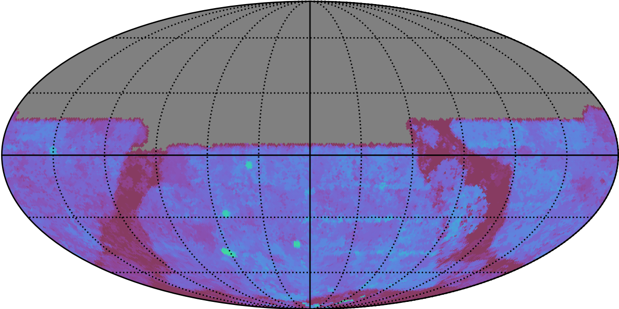
ddf_acor_sf10_lsf20_lsr20_v3.4_10yrs All sky u band: 80thPercentile Season Length
