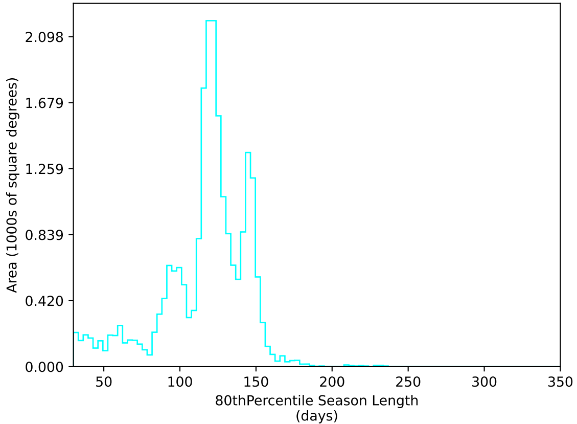
ddf_acor_sf10_lsf20_lsr20_v3.4_10yrs All sky u band: 80thPercentile Season Length
