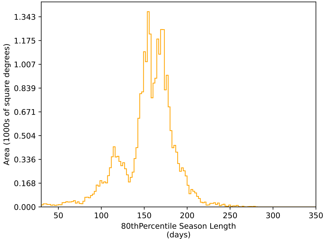
ddf_acor_sf10_lsf20_lsr20_v3.4_10yrs All sky r band: 80thPercentile Season Length
