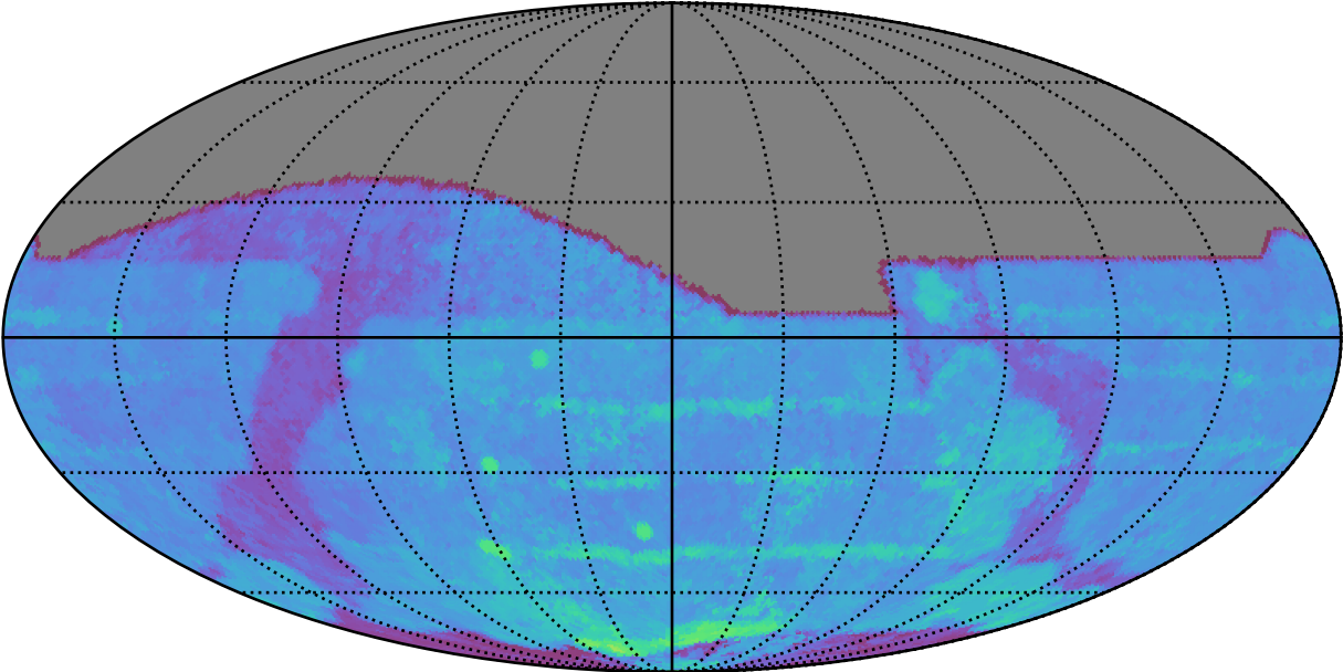
ddf_acor_sf10_lsf20_lsr20_v3.4_10yrs All sky i band: 80thPercentile Season Length
