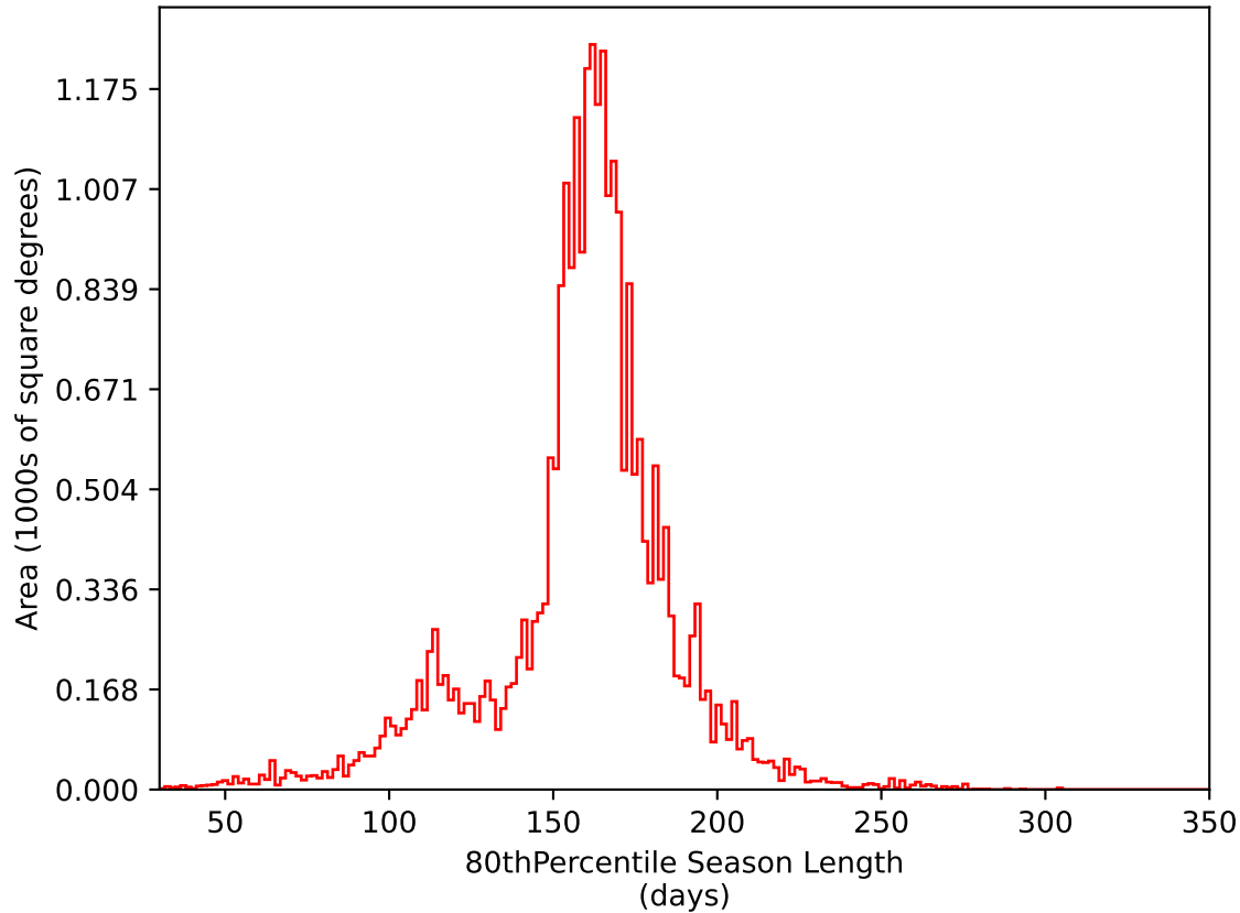
ddf_acor_sf10_lsf20_lsr20_v3.4_10yrs All sky i band: 80thPercentile Season Length
