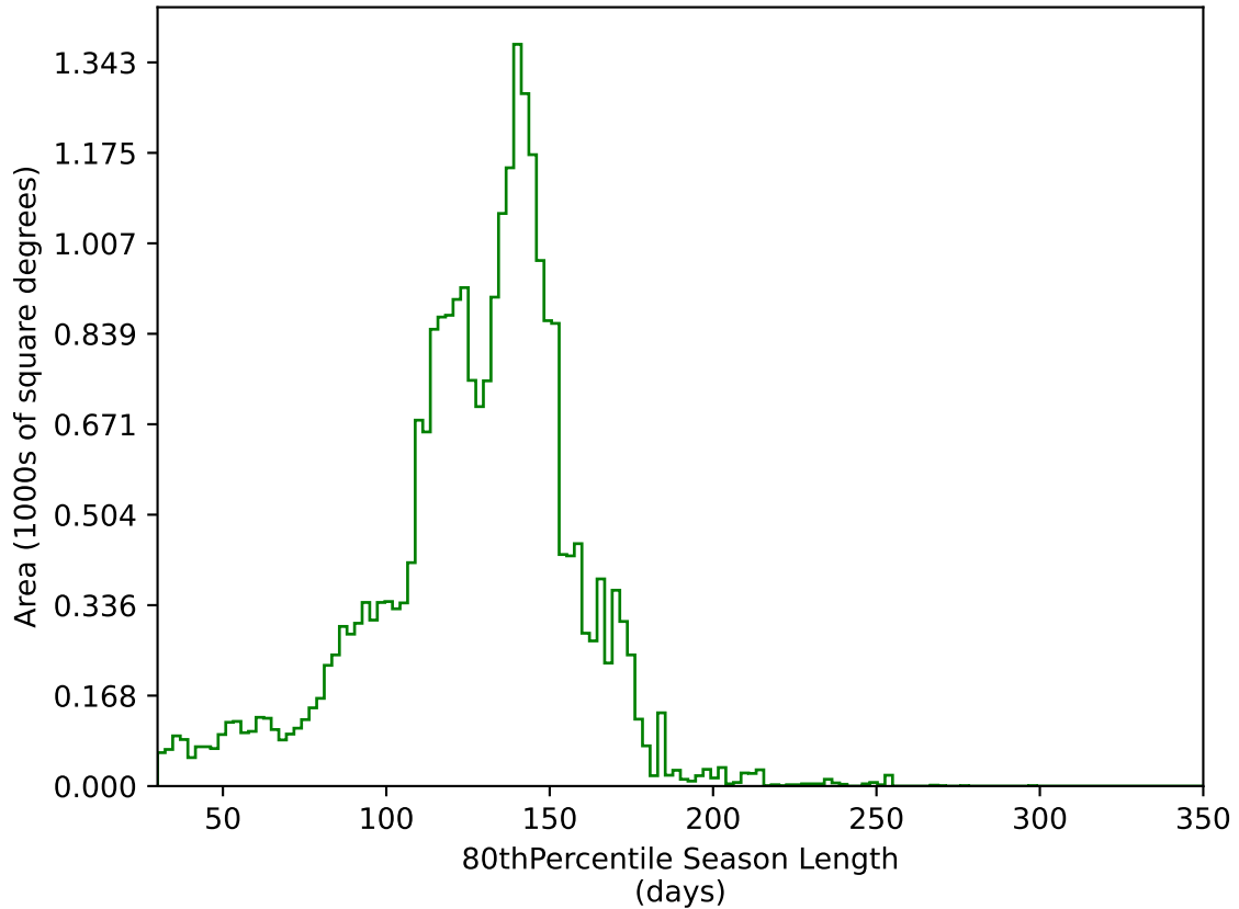
ddf_acor_sf10_lsf20_lsr20_v3.4_10yrs All sky g band: 80thPercentile Season Length
