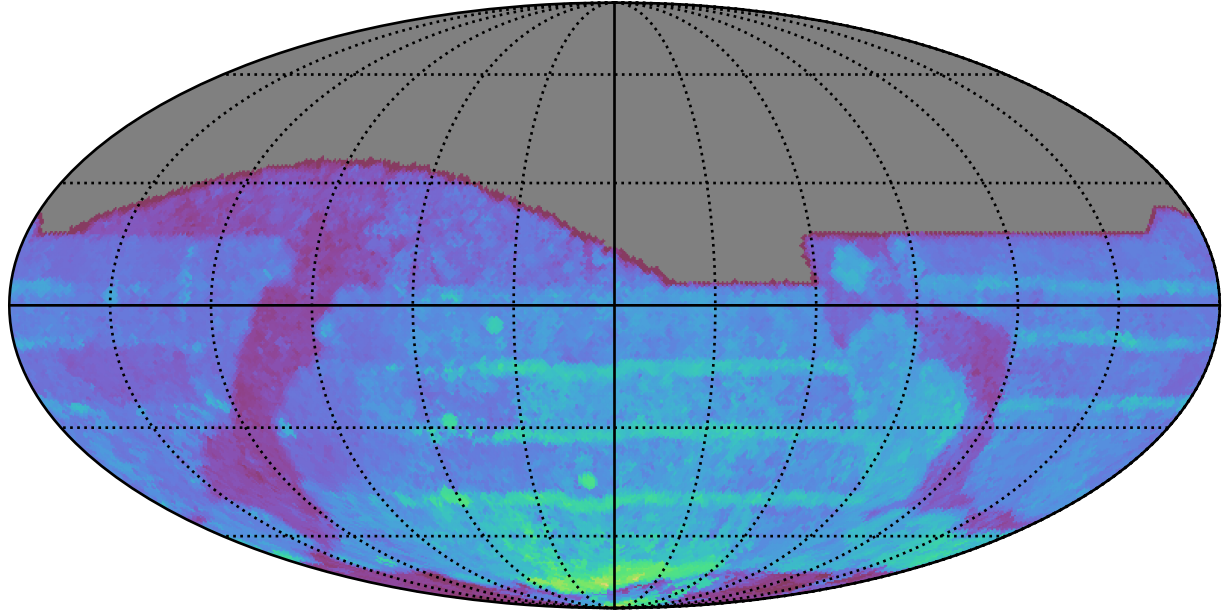
ddf_acor_sf10_lsf20_lsr20_v3.4_10yrs All sky all bands: 80thPercentile Season Length
