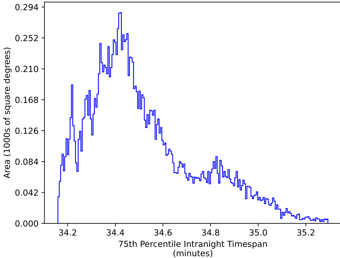
ddf_acor_sf10_lsf20_lsr20_v3.4_10yrs WFD zy bands: 75th Percentile Intranight Timespan
