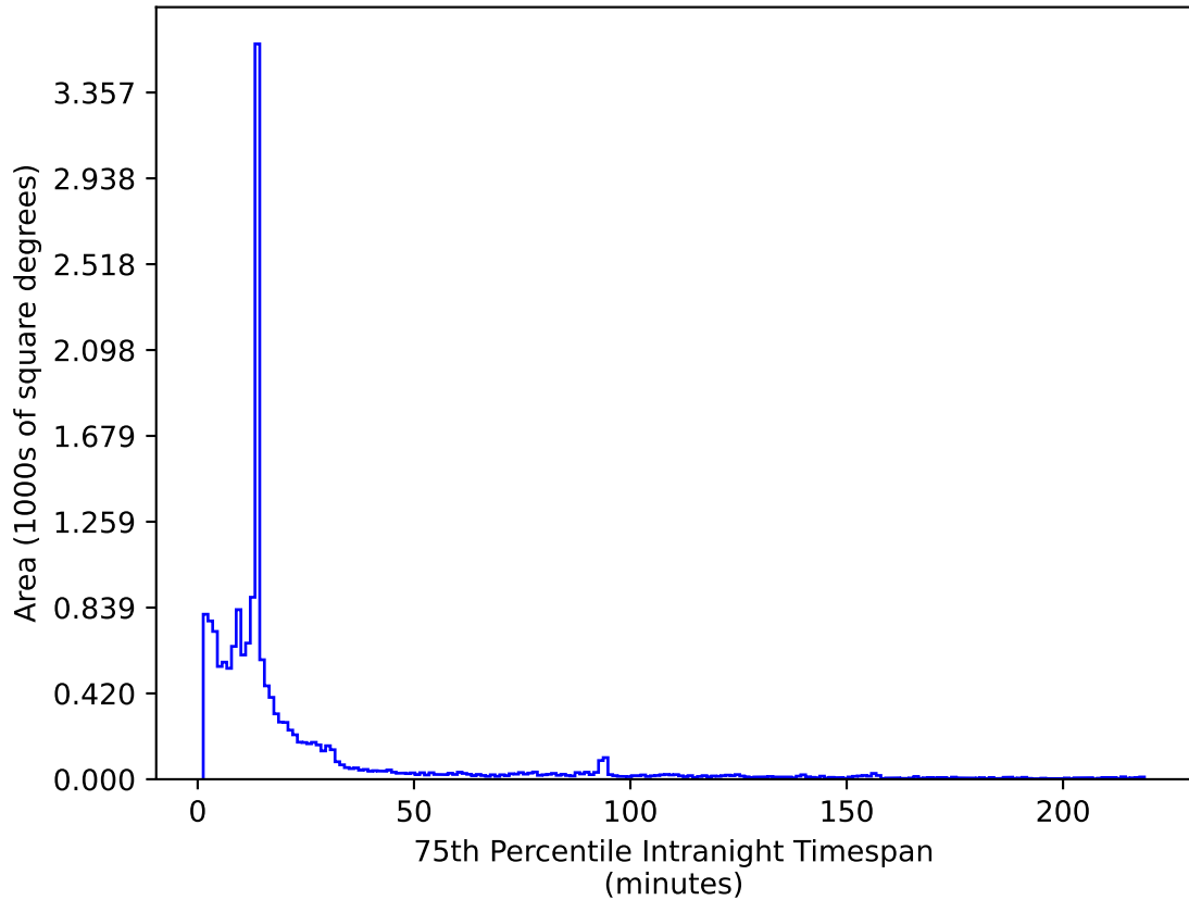
ddf_acor_sf10_lsf20_lsr20_v3.4_10yrs WFD z band: 75th Percentile Intranight Timespan
