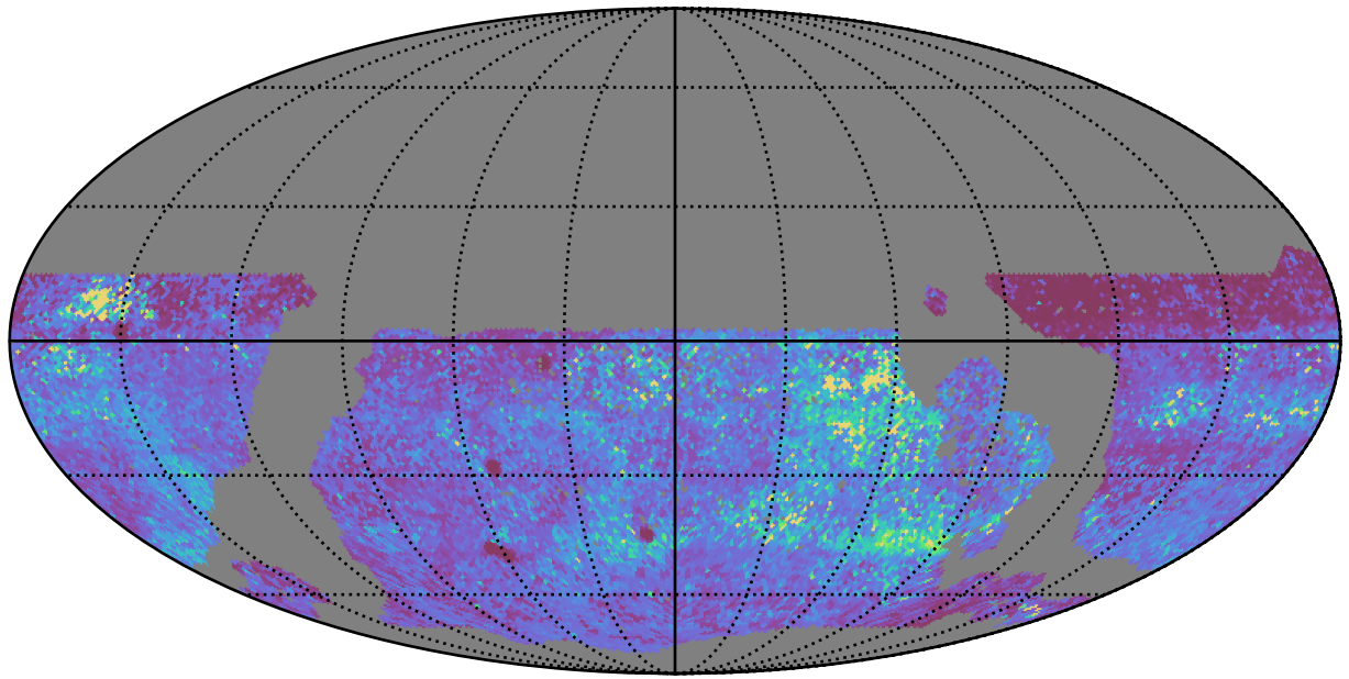
ddf_acor_sf10_lsf20_lsr20_v3.4_10yrs WFD y band: 75th Percentile Intranight Timespan
