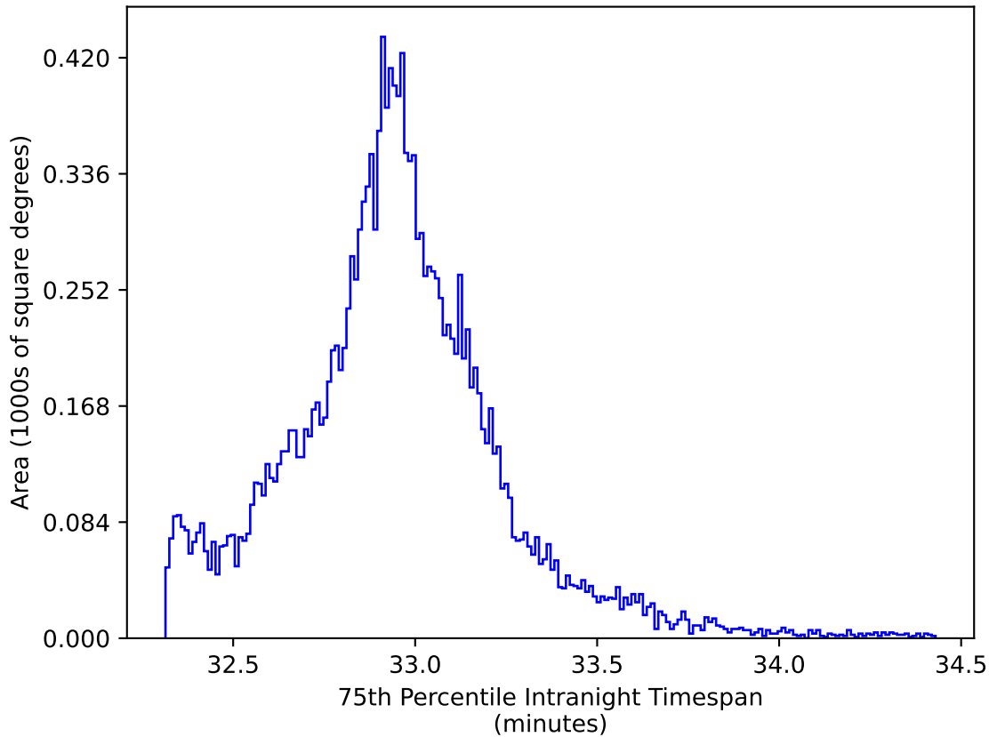
ddf_acor_sf10_lsf20_lsr20_v3.4_10yrs WFD y band: 75th Percentile Intranight Timespan
