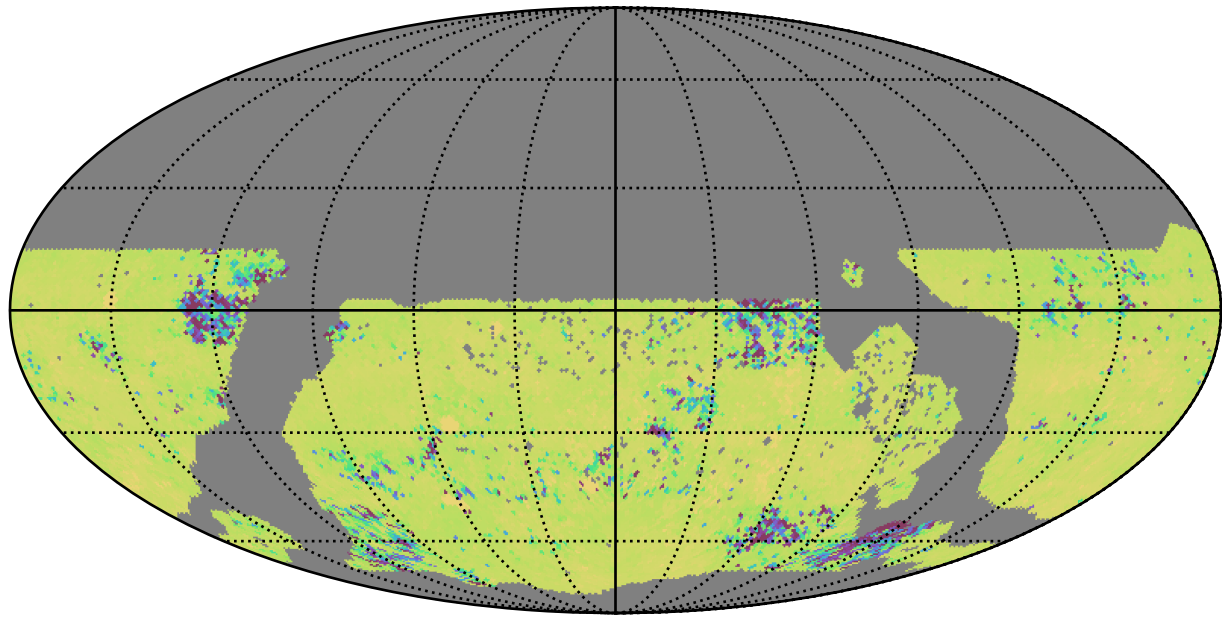
ddf_acor_sf10_lsf20_lsr20_v3.4_10yrs WFD ug bands: 75th Percentile Intranight Timespan
