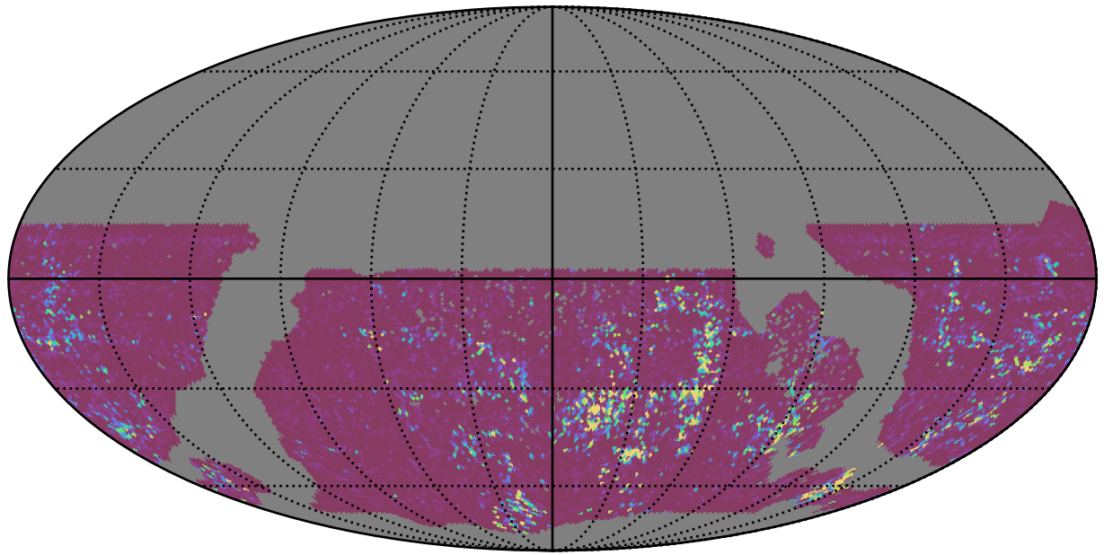
ddf_acor_sf10_lsf20_lsr20_v3.4_10yrs WFD u band: 75th Percentile Intranight Timespan
