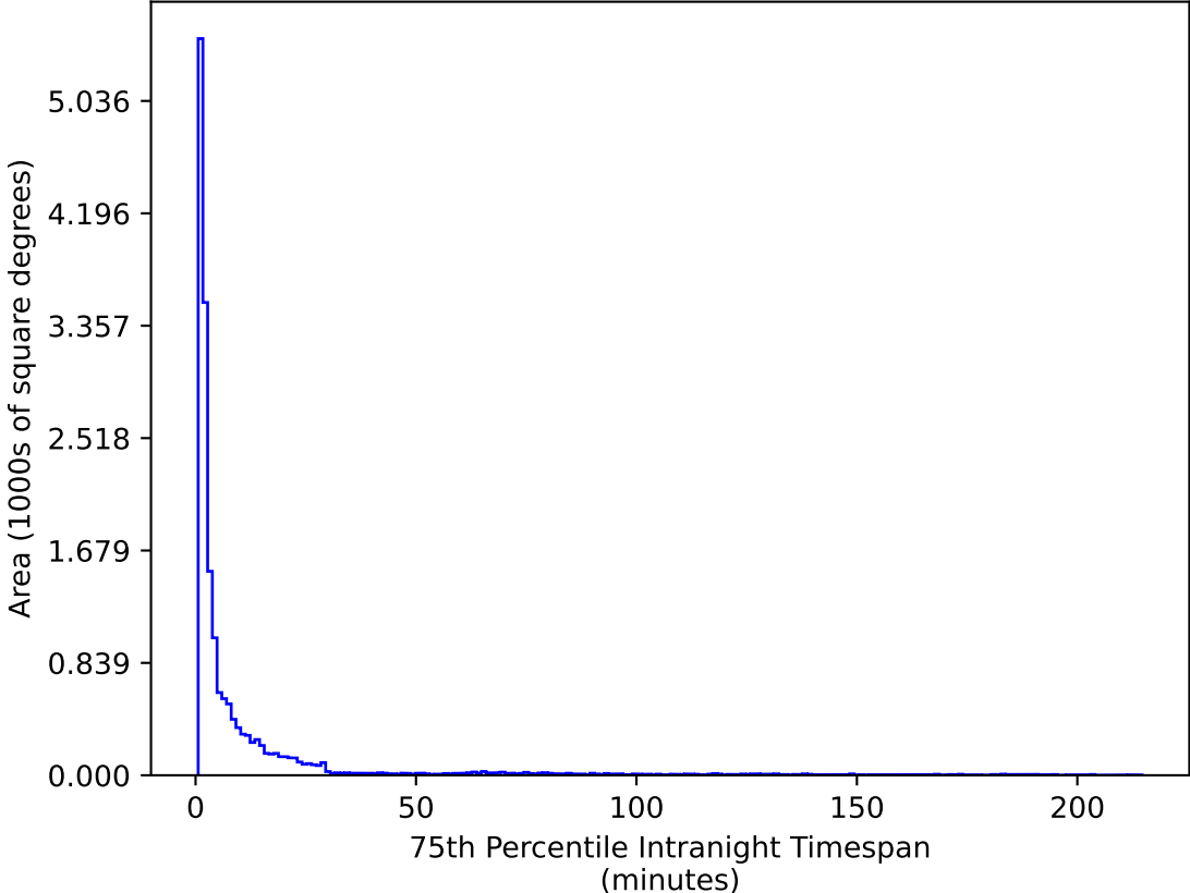
ddf_acor_sf10_lsf20_lsr20_v3.4_10yrs WFD u band: 75th Percentile Intranight Timespan
