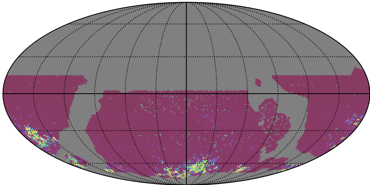
ddf_acor_sf10_lsf20_lsr20_v3.4_10yrs WFD ri bands: 75th Percentile Intranight Timespan
