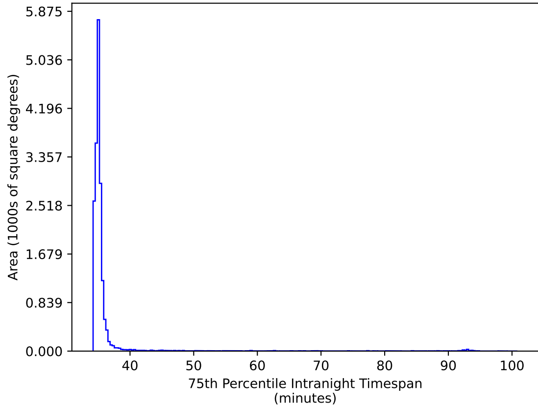
ddf_acor_sf10_lsf20_lsr20_v3.4_10yrs WFD ri bands: 75th Percentile Intranight Timespan
