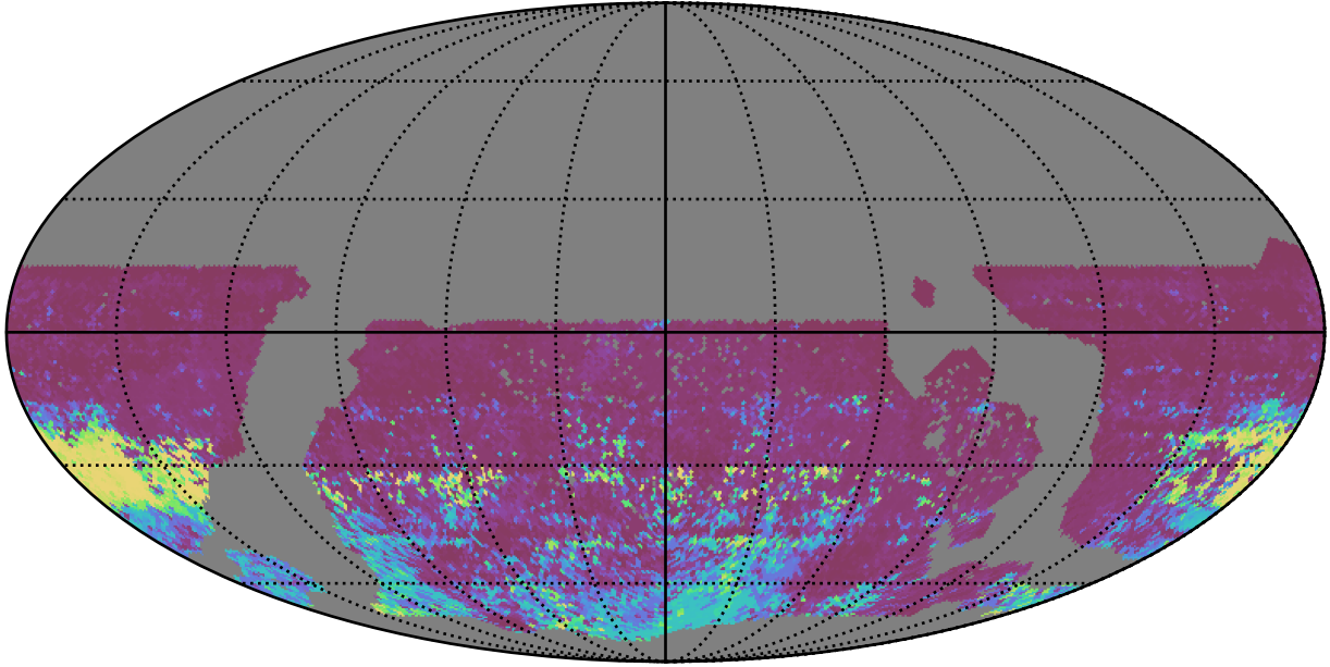
ddf_acor_sf10_lsf20_lsr20_v3.4_10yrs WFD r band: 75th Percentile Intranight Timespan
