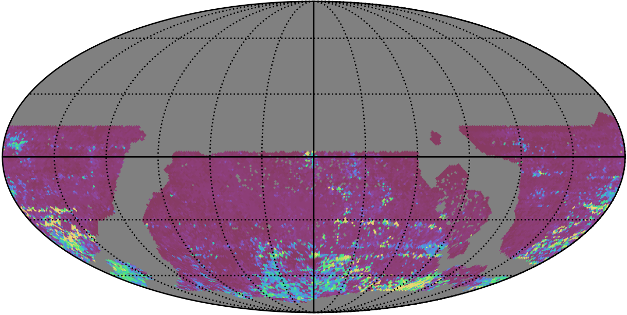
ddf_acor_sf10_lsf20_lsr20_v3.4_10yrs WFD i band: 75th Percentile Intranight Timespan
