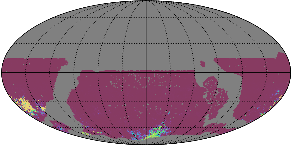
ddf_acor_sf10_lsf20_lsr20_v3.4_10yrs WFD gr bands: 75th Percentile Intranight Timespan
