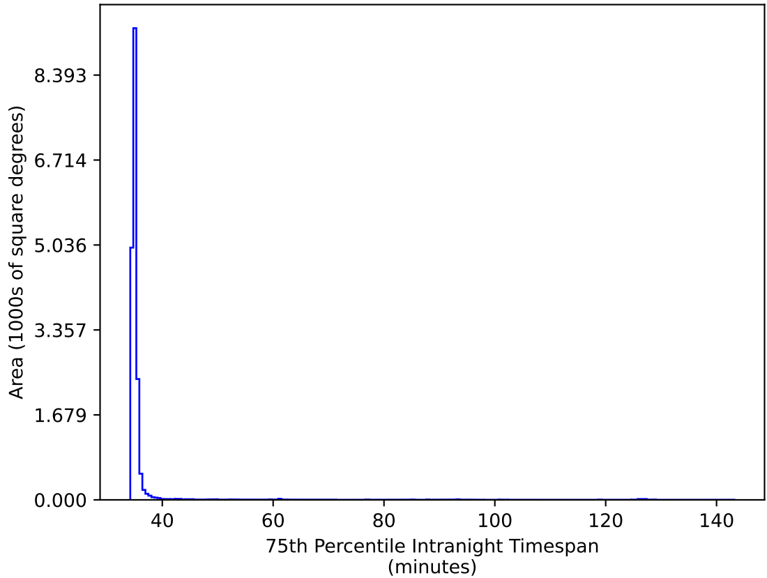
ddf_acor_sf10_lsf20_lsr20_v3.4_10yrs WFD gr bands: 75th Percentile Intranight Timespan
