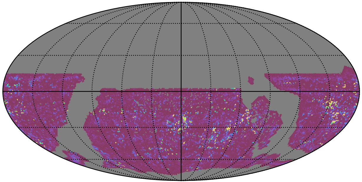
ddf_acor_sf10_lsf20_lsr20_v3.4_10yrs WFD g band: 75th Percentile Intranight Timespan
