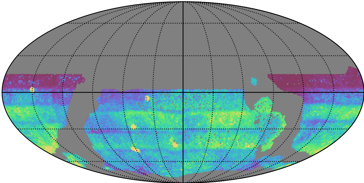
ddf_acor_sf10_lsf20_lsr20_v3.4_10yrs WFD: 75th Percentile Intranight Timespan
