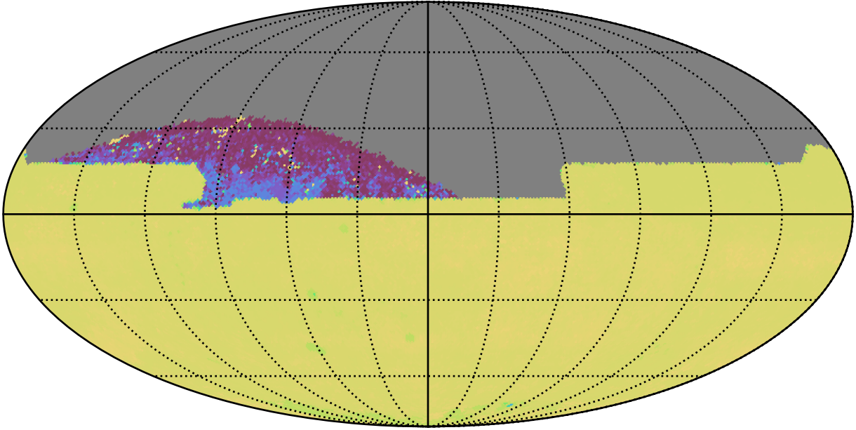
ddf_acor_sf10_lsf20_lsr20_v3.4_10yrs All sky zy bands: 75th Percentile Intranight Timespan
