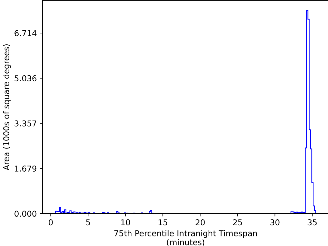
ddf_acor_sf10_lsf20_lsr20_v3.4_10yrs All sky zy bands: 75th Percentile Intranight Timespan
