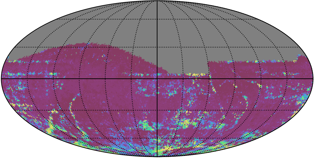
ddf_acor_sf10_lsf20_lsr20_v3.4_10yrs All sky z band: 75th Percentile Intranight Timespan
