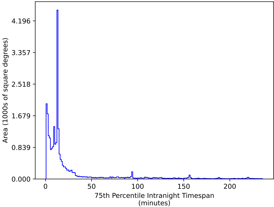
ddf_acor_sf10_lsf20_lsr20_v3.4_10yrs All sky z band: 75th Percentile Intranight Timespan
