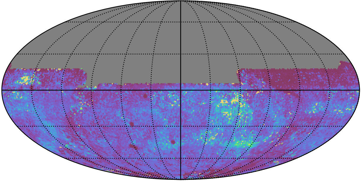
ddf_acor_sf10_lsf20_lsr20_v3.4_10yrs All sky y band: 75th Percentile Intranight Timespan
